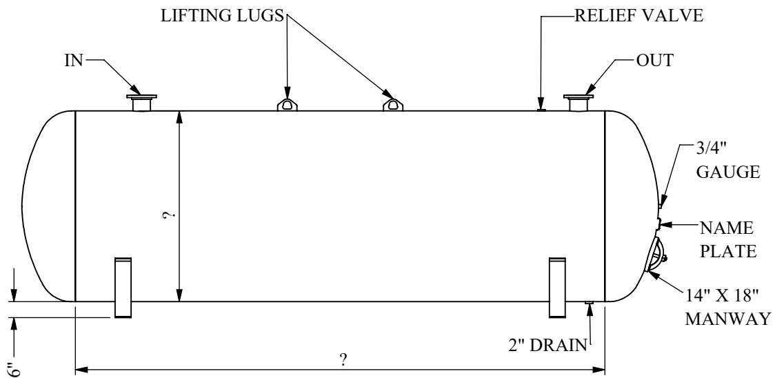
HORIZONTAL SPRINKLER TANK
